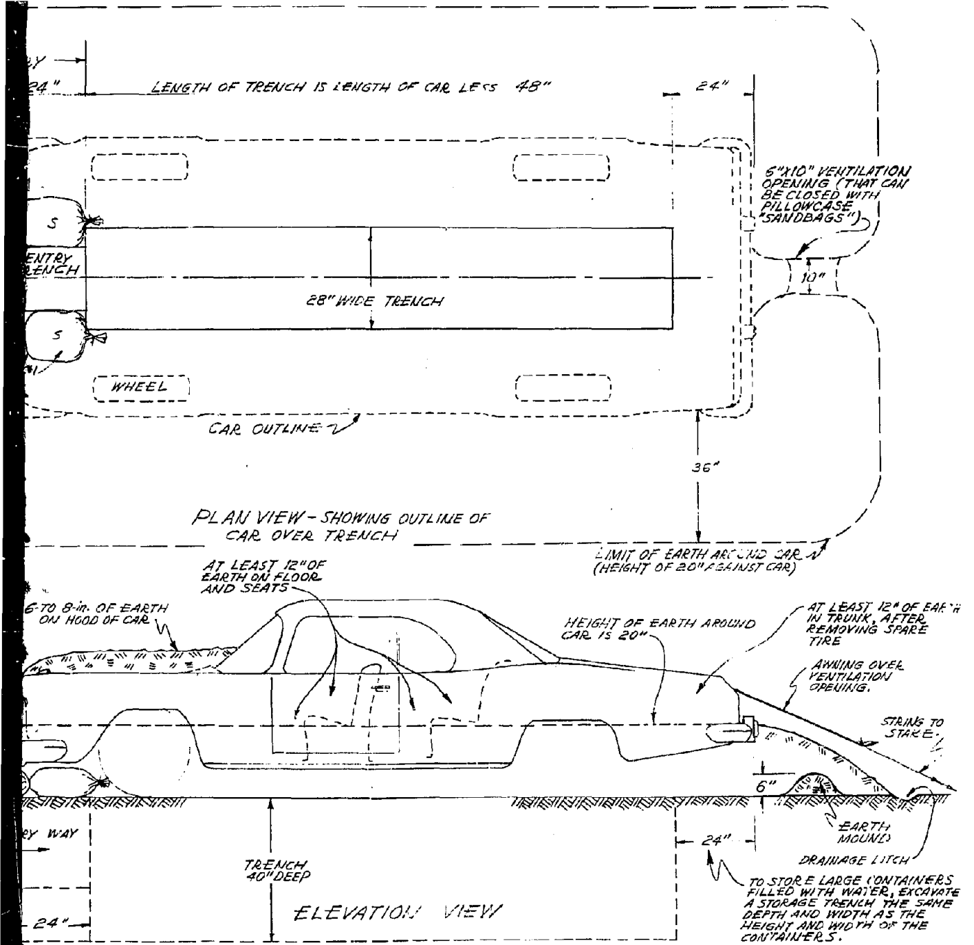
Fig. A-13.2. Car-Over-Trench Shelter, Plan and Elevation.
